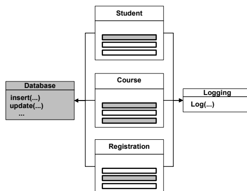
Figure 3.1: Code tangling example [cod]
