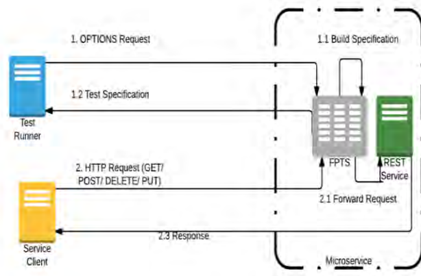
Figure 8: Framework Behavior for HTTP Requests [13]
