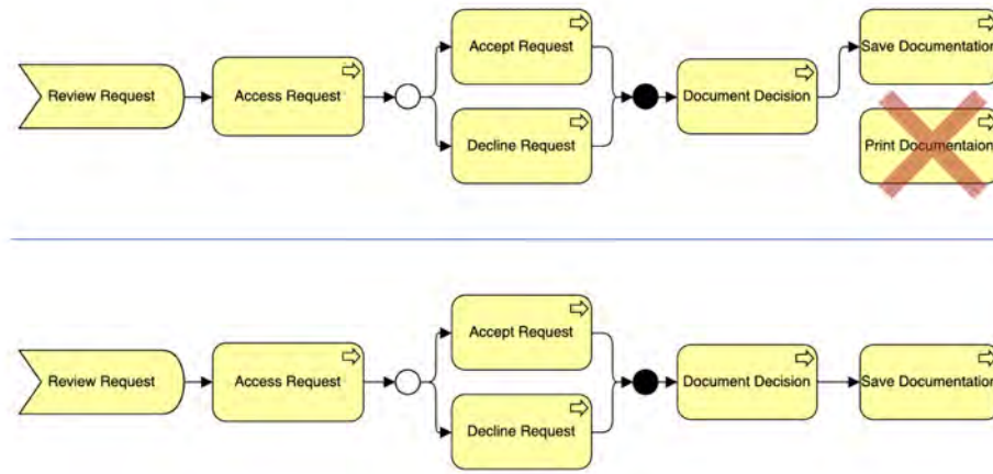
Figure 3: EA refactoring: Remove Dead Component
