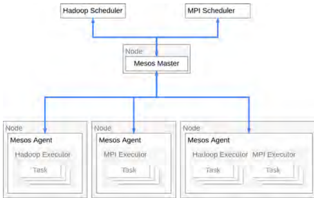
Figure 1: Cluster Architecture of Mesos
