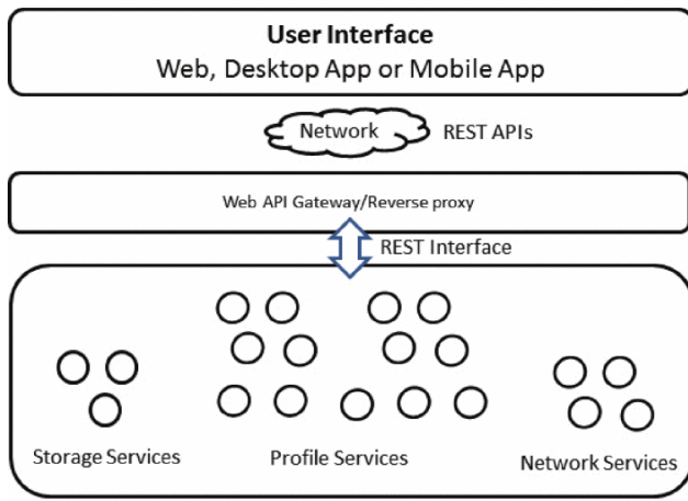
Figure 1: An example structure using REST API [6]
