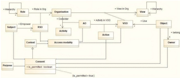
Figure 3: PrivUML meta-model [18]
