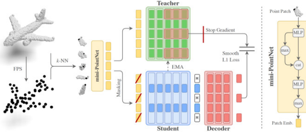
Figure 10: Input Data, Masked Data and Further Explained Components. Taken From [20]
