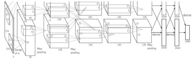
Figure 11: Data-Oriented Visualization of a CNN-Architecture. Taken From [23]
