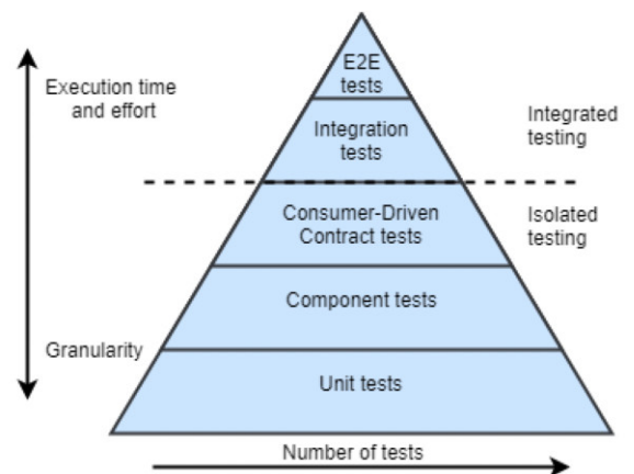
Figure 2: Test pyramid with consumer-driven contract tests. Adapted from [5]
